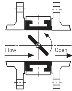
Preferred mounting
